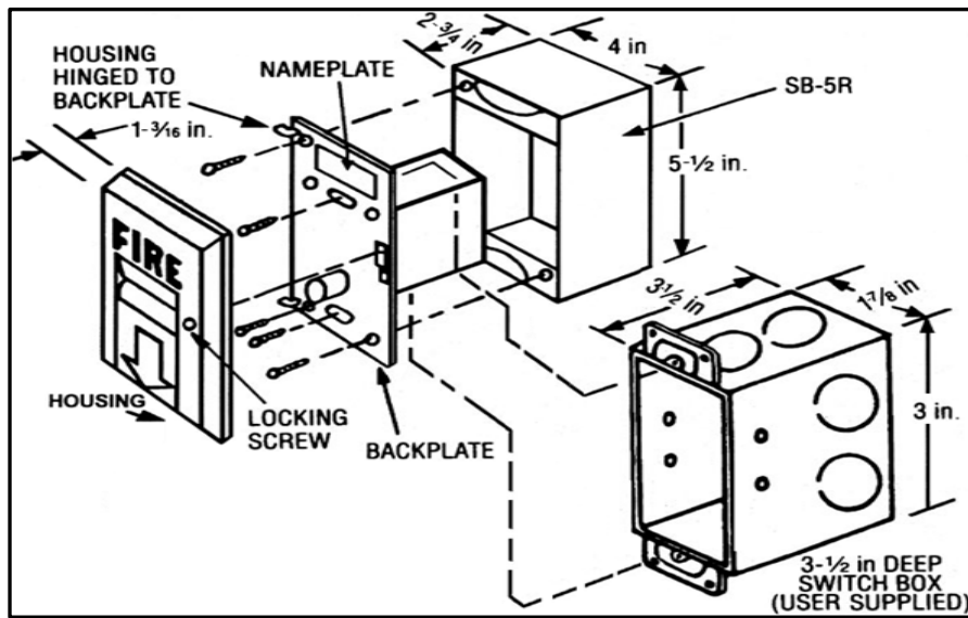
Mounting Diagram
